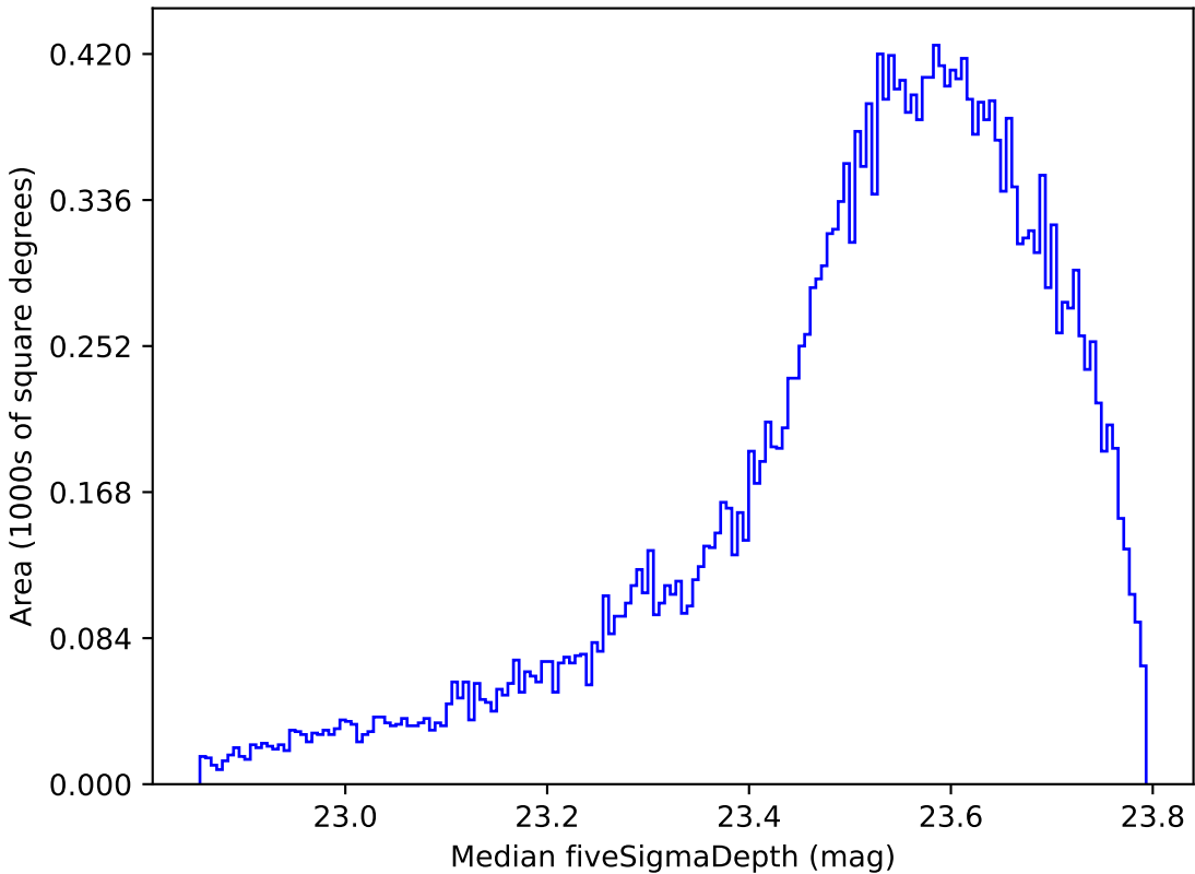
too_ignore_10_4v3.4_10yrs All sky i band: Median fiveSigmaDepth
