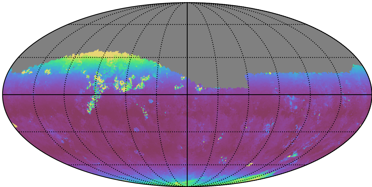
too_ignore_10_4v3.4_10yrs Yr 1 z band: Median airmass
