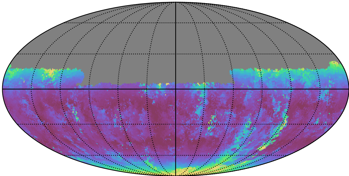
too_ignore_10_4v3.4_10yrs Yr 1 u band: Median airmass
