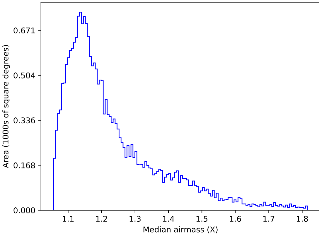
too_ignore_10_4v3.4_10yrs Yr 1 u band: Median airmass
