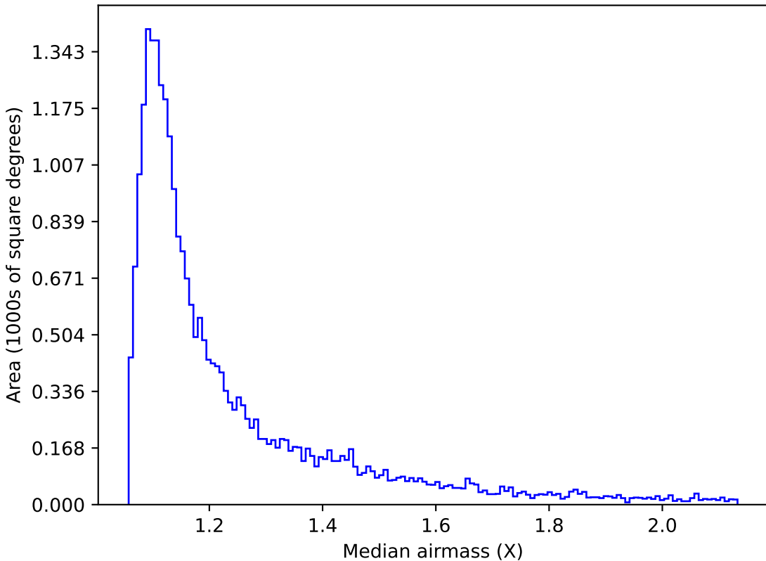
too_ignore_10_4v3.4_10yrs Yr 1 r band: Median airmass
