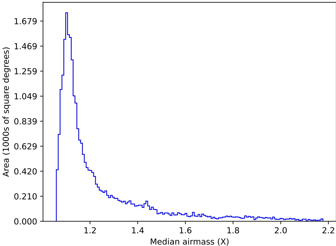
too_ignore_10_4v3.4_10yrs Yr 1 i band: Median airmass
