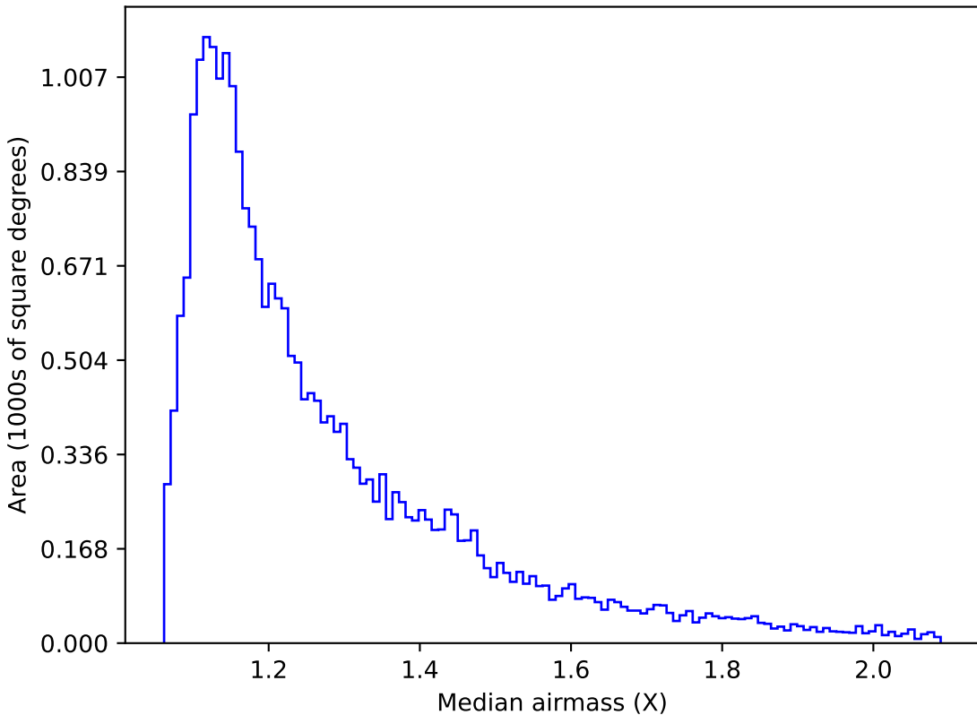
too_ignore_10_4v3.4_10yrs Yr 1 g band: Median airmass
