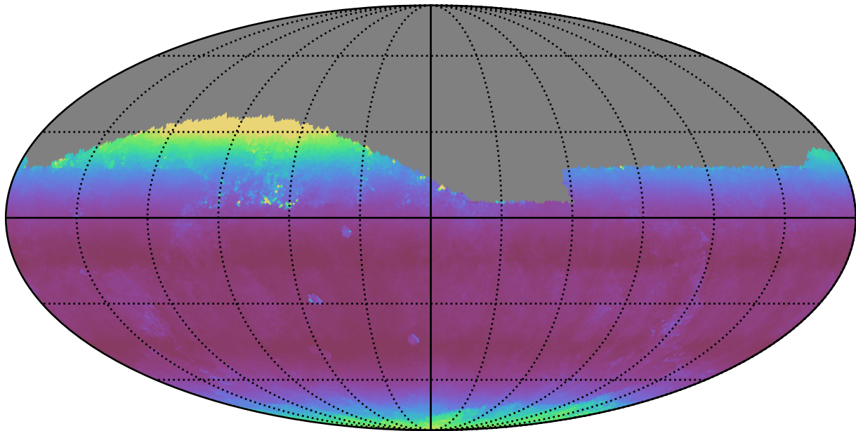
too_ignore_10_4v3.4_10yrs Yr 1 all bands: Median airmass
