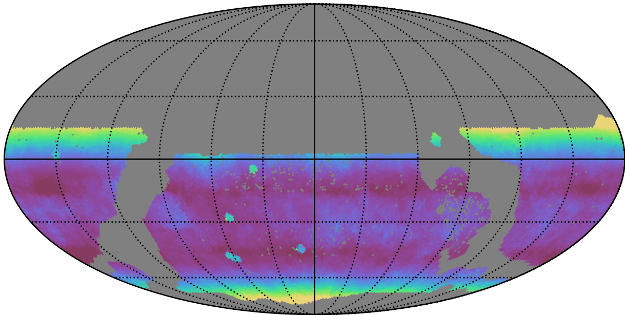
too_ignore_10_4v3.4_10yrs WFD z band: Median airmass
