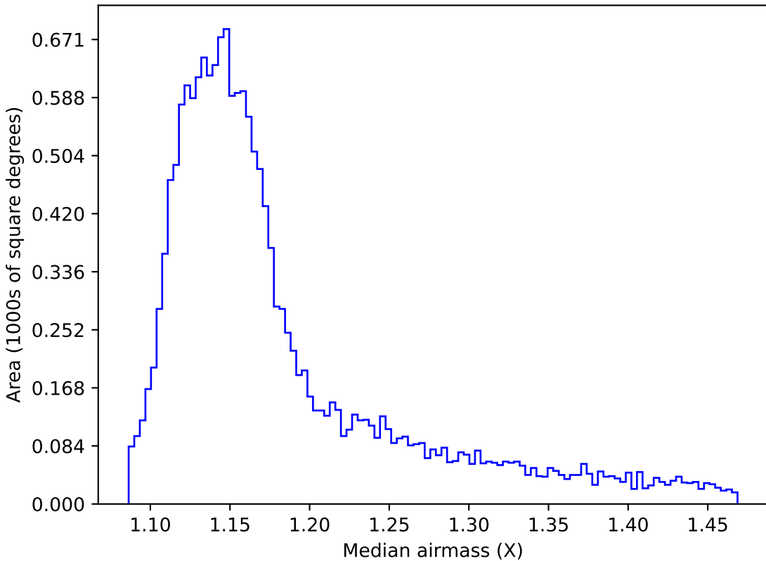
too_ignore_10_4v3.4_10yrs WFD z band: Median airmass
