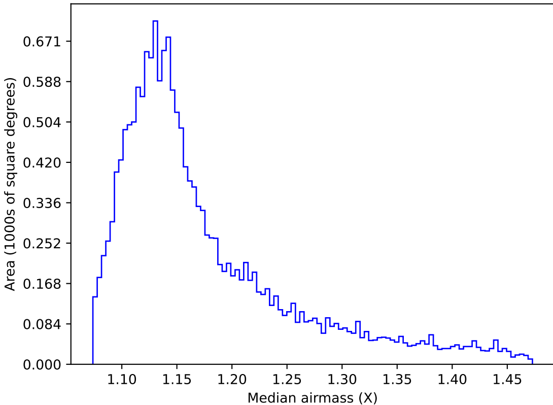
too_ignore_10_4v3.4_10yrs WFD u band: Median airmass
