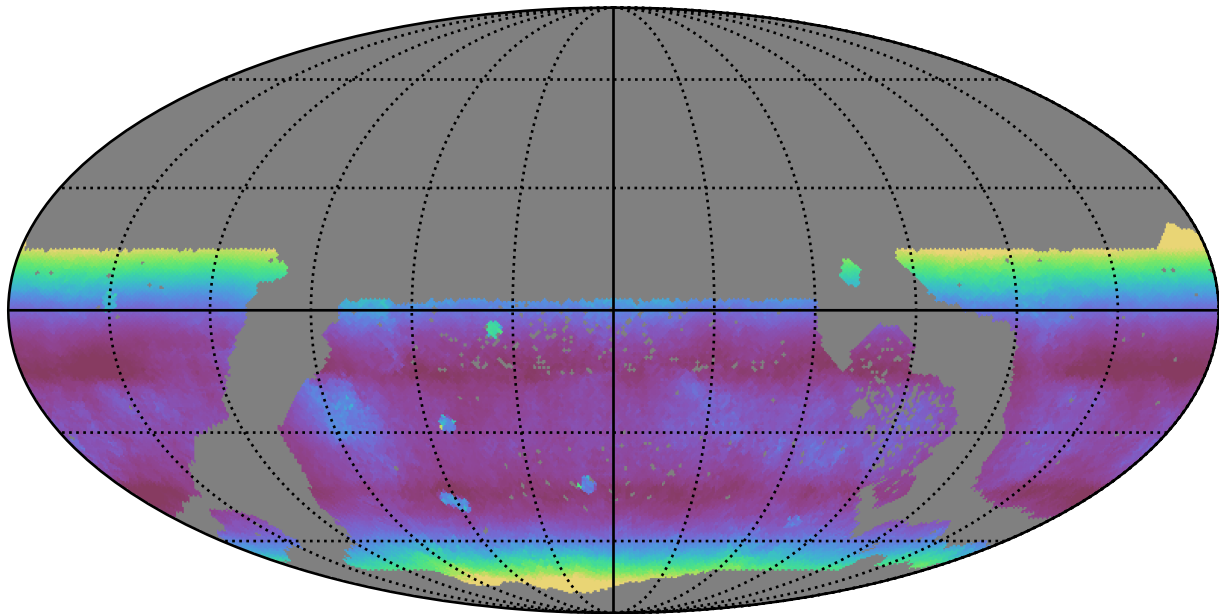
too_ignore_10_4v3.4_10yrs WFD r band: Median airmass
