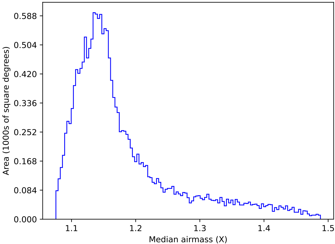
too_ignore_10_4v3.4_10yrs WFD g band: Median airmass
