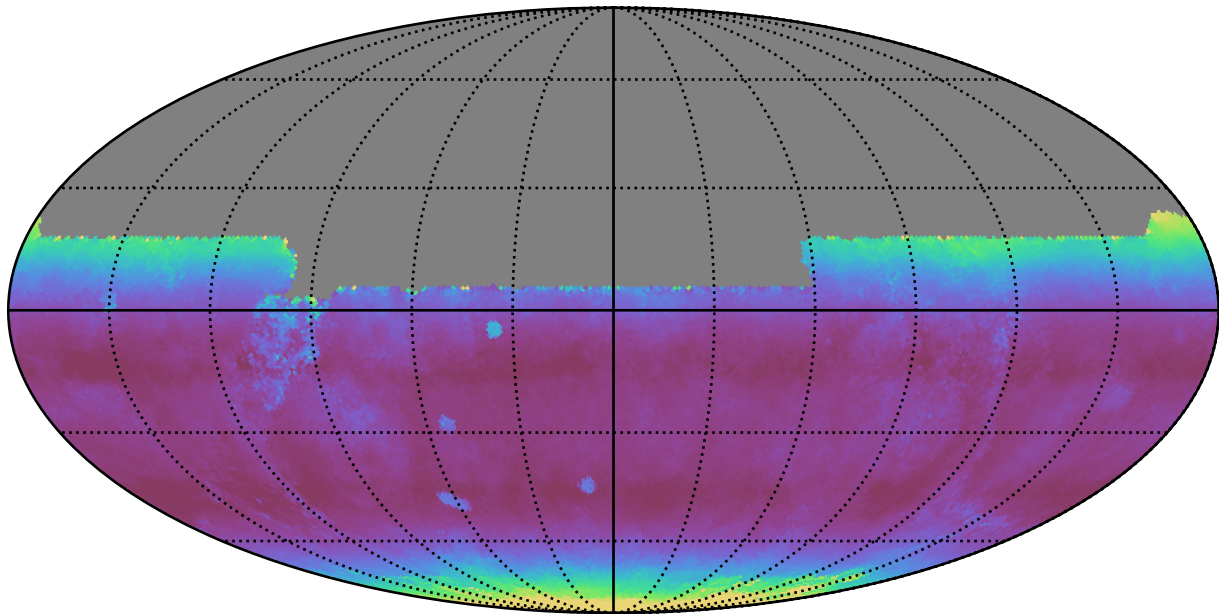
too_ignore_10_4v3.4_10yrs All sky y band: Median airmass
