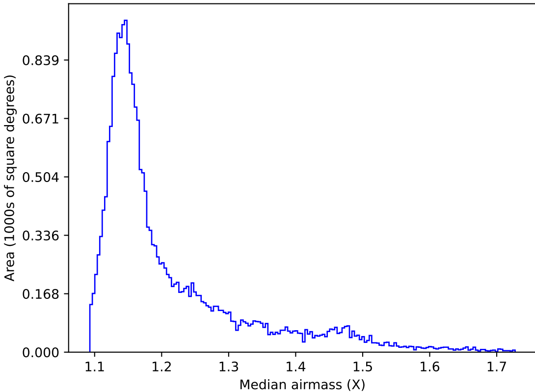
too_ignore_10_4v3.4_10yrs All sky y band: Median airmass
