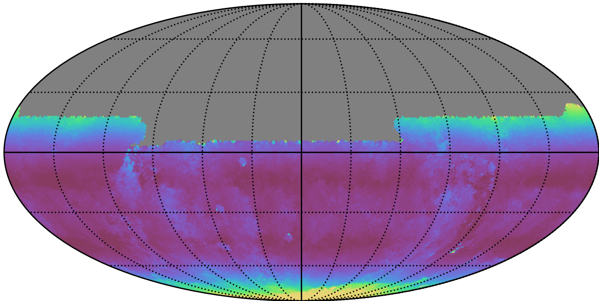
too_ignore_10_4v3.4_10yrs All sky u band: Median airmass
