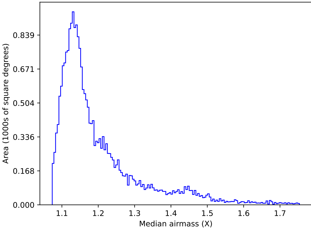
too_ignore_10_4v3.4_10yrs All sky u band: Median airmass
