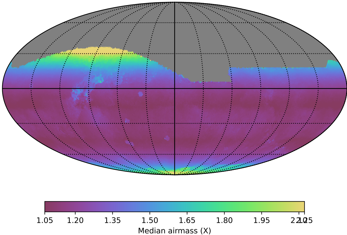
too_ignore_10_4v3.4_10yrs All sky r band: Median airmass
