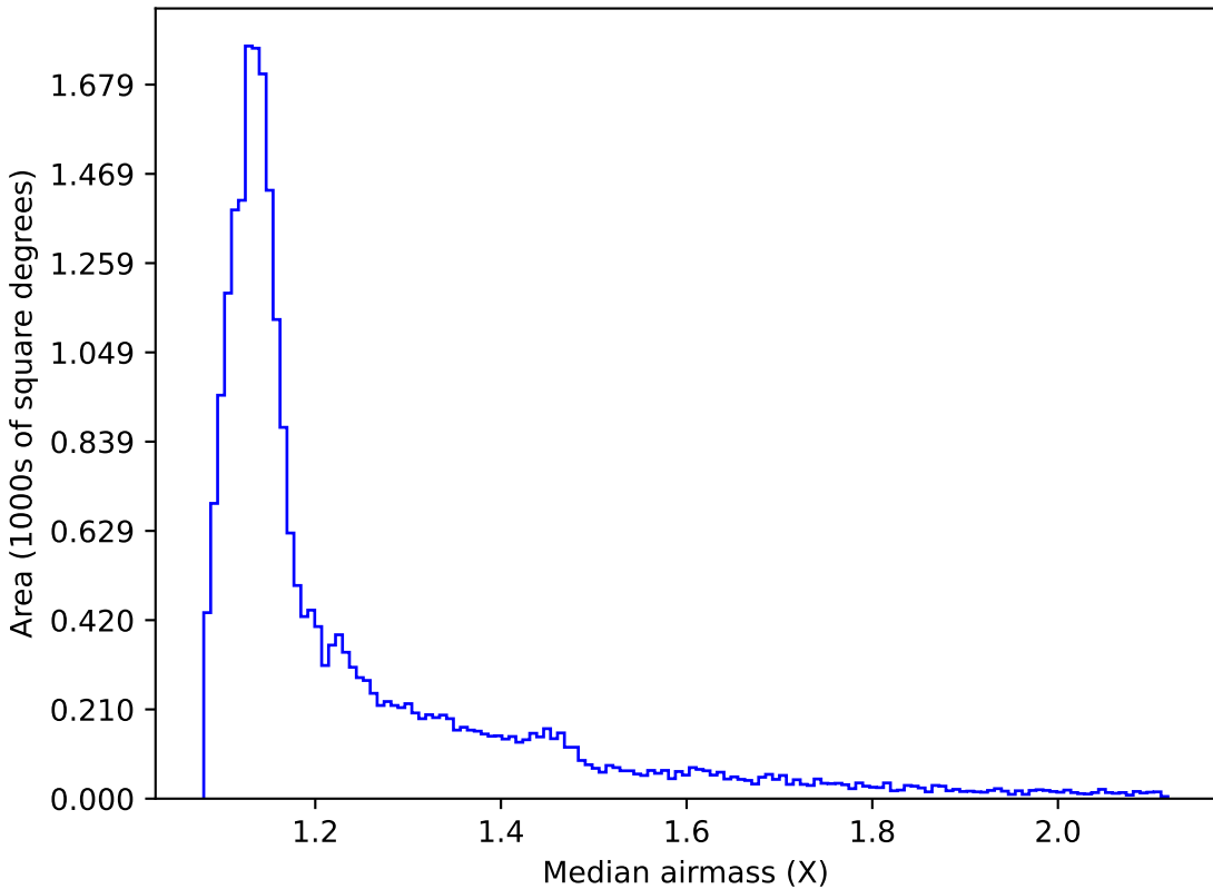
too_ignore_10_4v3.4_10yrs All sky i band: Median airmass
