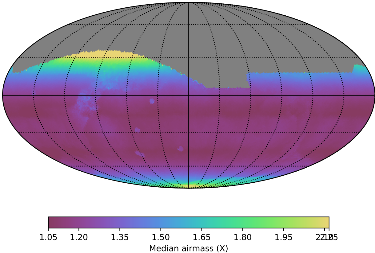
too_ignore_10_4v3.4_10yrs All sky all bands: Median airmass
