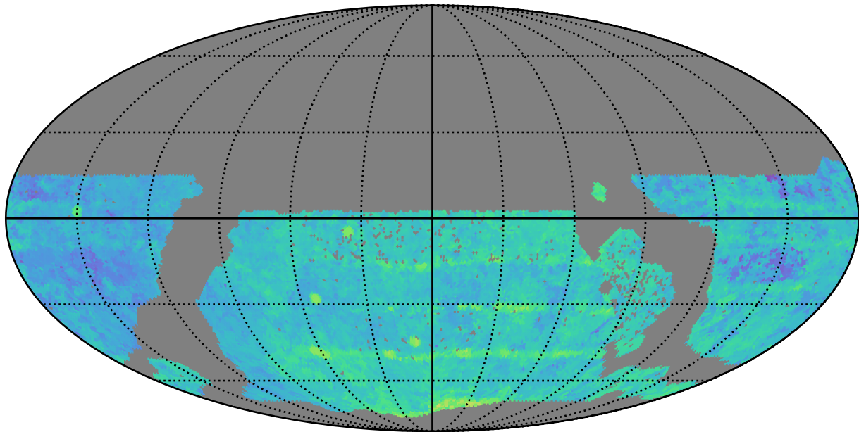
too_ignore_10_4v3.4_10yrs WFD z band: Median Season Length
