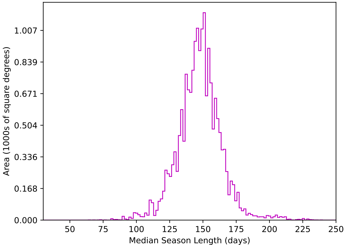
too_ignore_10_4v3.4_10yrs WFD z band: Median Season Length
