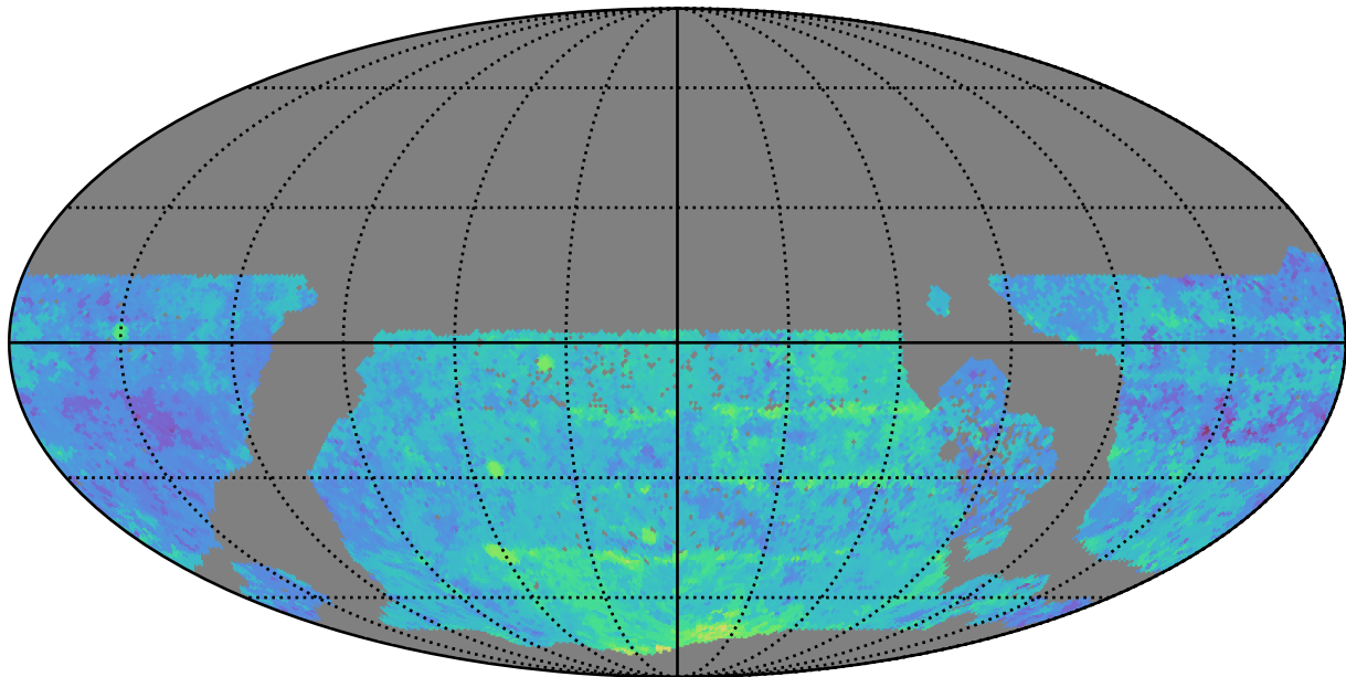
too_ignore_10_4v3.4_10yrs WFD y band: Median Season Length
