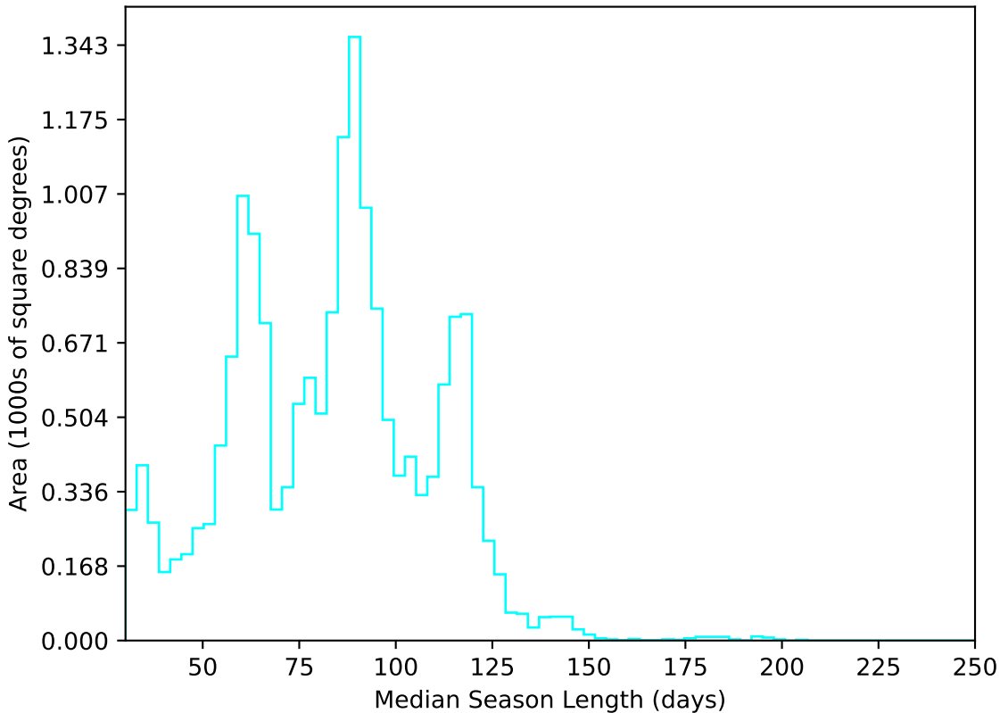
too_ignore_10_4v3.4_10yrs WFD u band: Median Season Length
