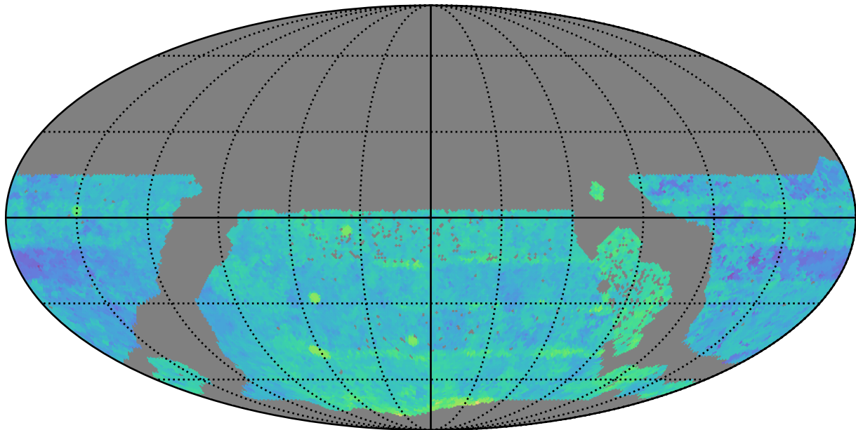
too_ignore_10_4v3.4_10yrs WFD i band: Median Season Length
