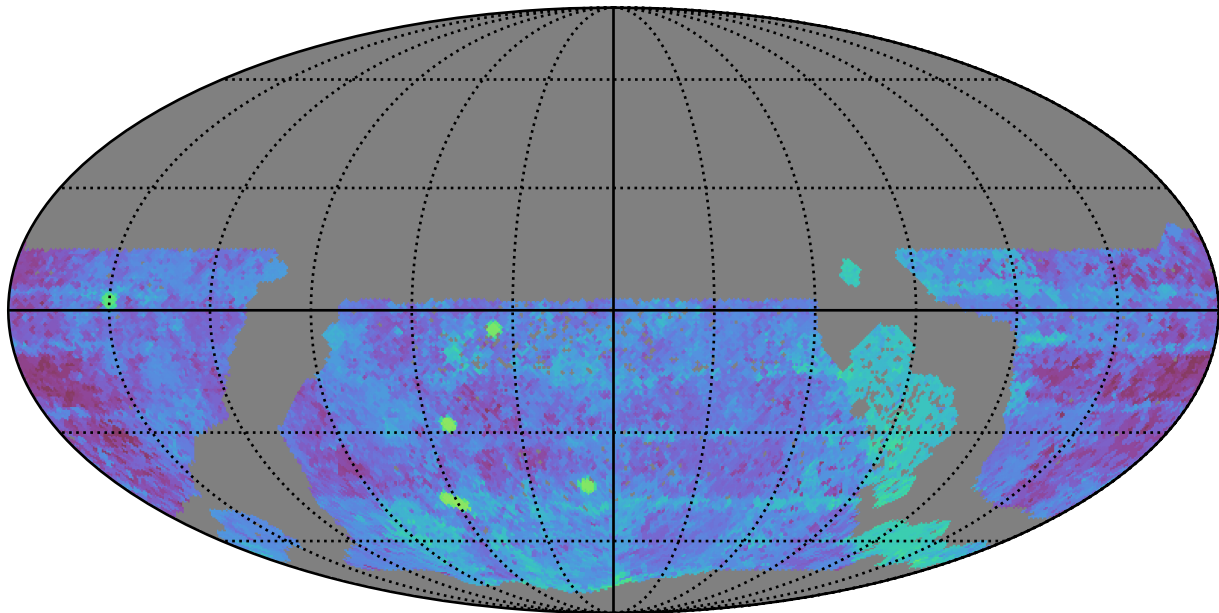
too_ignore_10_4v3.4_10yrs WFD g band: Median Season Length
