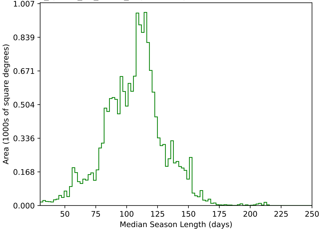
too_ignore_10_4v3.4_10yrs WFD g band: Median Season Length
