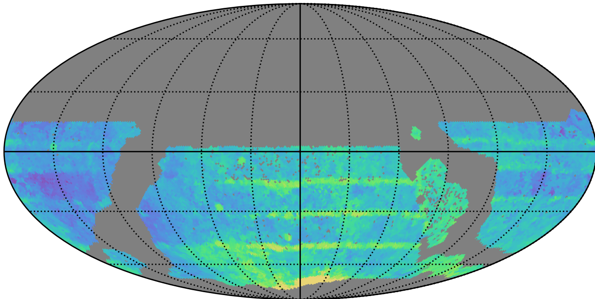
too_ignore_10_4v3.4_10yrs WFD all bands: Median Season Length
