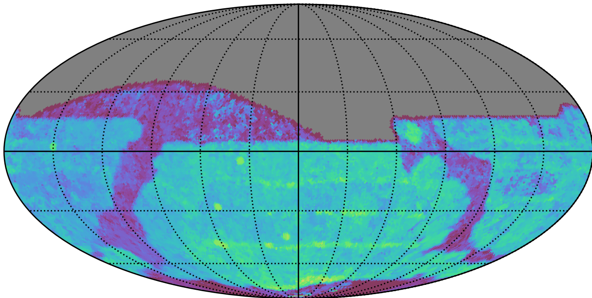
too_ignore_10_4v3.4_10yrs All sky z band: Median Season Length
