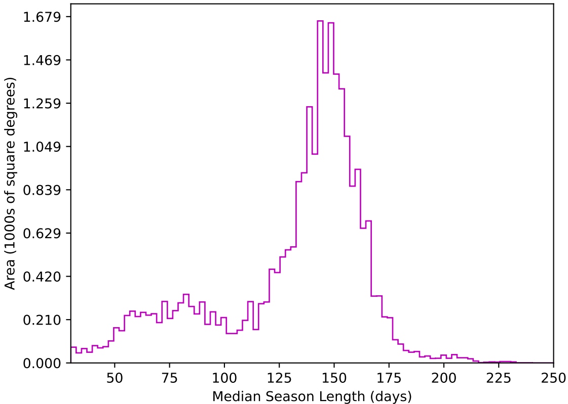
too_ignore_10_4v3.4_10yrs All sky z band: Median Season Length
