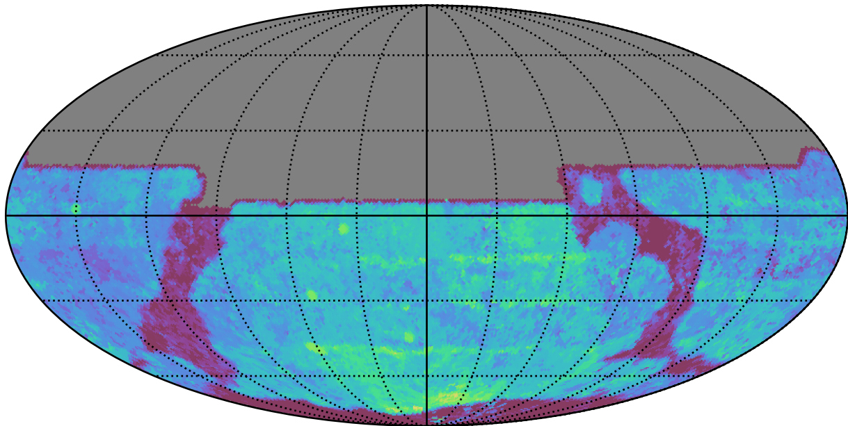
too_ignore_10_4v3.4_10yrs All sky y band: Median Season Length
