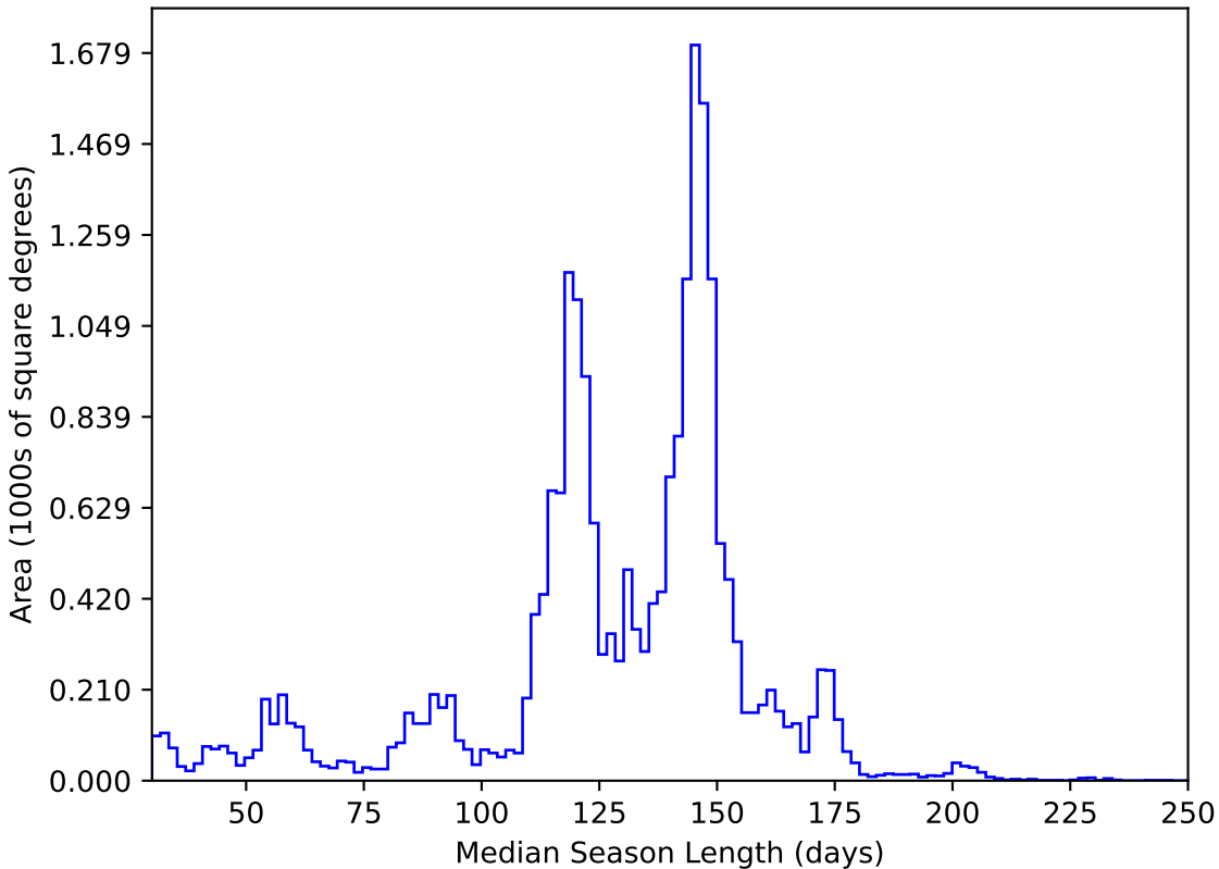
too_ignore_10_4v3.4_10yrs All sky y band: Median Season Length
