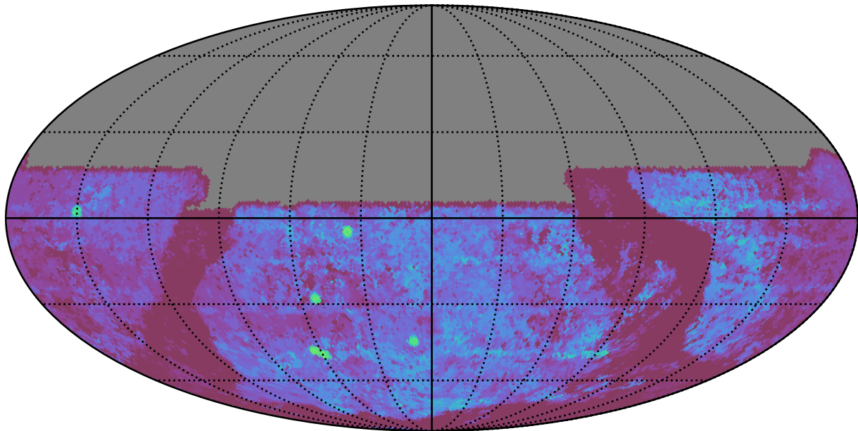
too_ignore_10_4v3.4_10yrs All sky u band: Median Season Length
