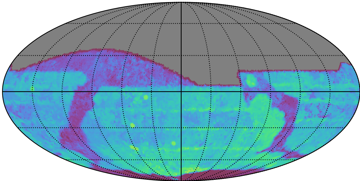
too_ignore_10_4v3.4_10yrs All sky r band: Median Season Length
