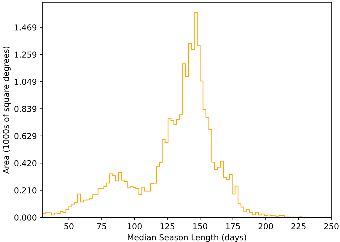
too_ignore_10_4v3.4_10yrs All sky r band: Median Season Length
