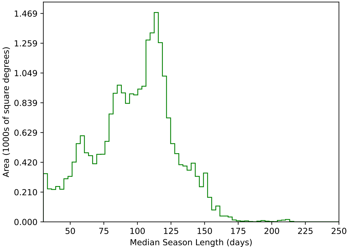
too_ignore_10_4v3.4_10yrs All sky g band: Median Season Length
