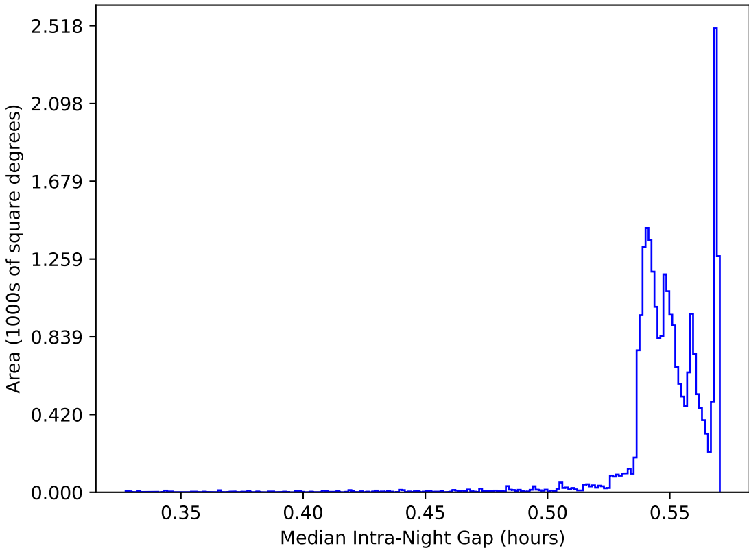
too_ignore_10_4v3.4_10yrs All sky: Median Intra-Night Gap
