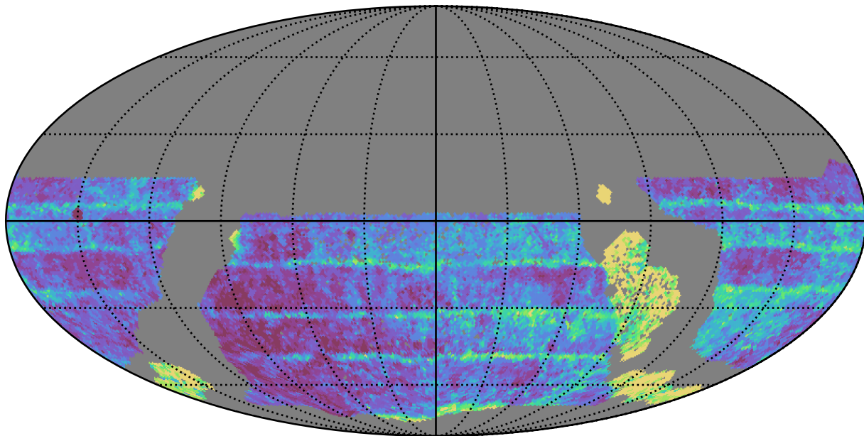
too_ignore_10_4v3.4_10yrs WFD z band: Median Inter-Night Gap
