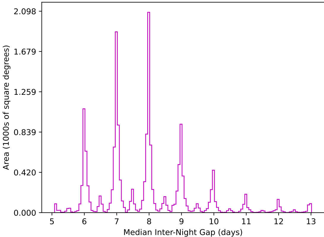
too_ignore_10_4v3.4_10yrs WFD z band: Median Inter-Night Gap
