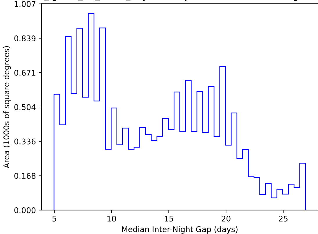
too_ignore_10_4v3.4_10yrs WFD y band: Median Inter-Night Gap
