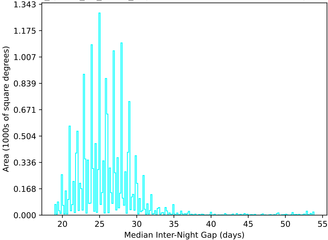
too_ignore_10_4v3.4_10yrs WFD u band: Median Inter-Night Gap
