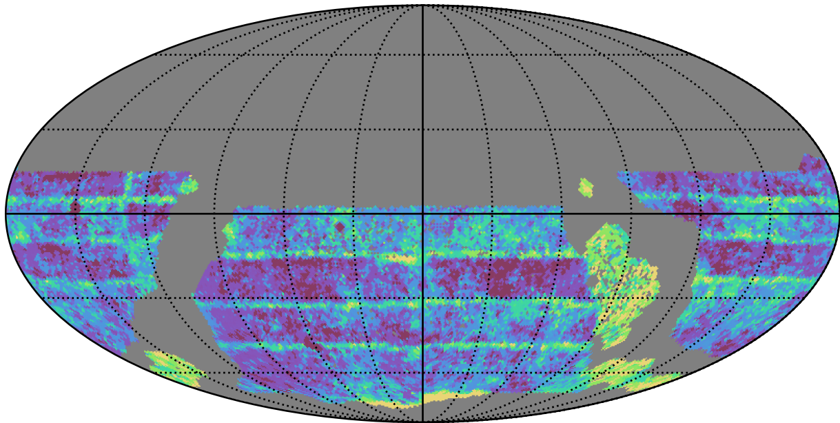
too_ignore_10_4v3.4_10yrs WFD i band: Median Inter-Night Gap
