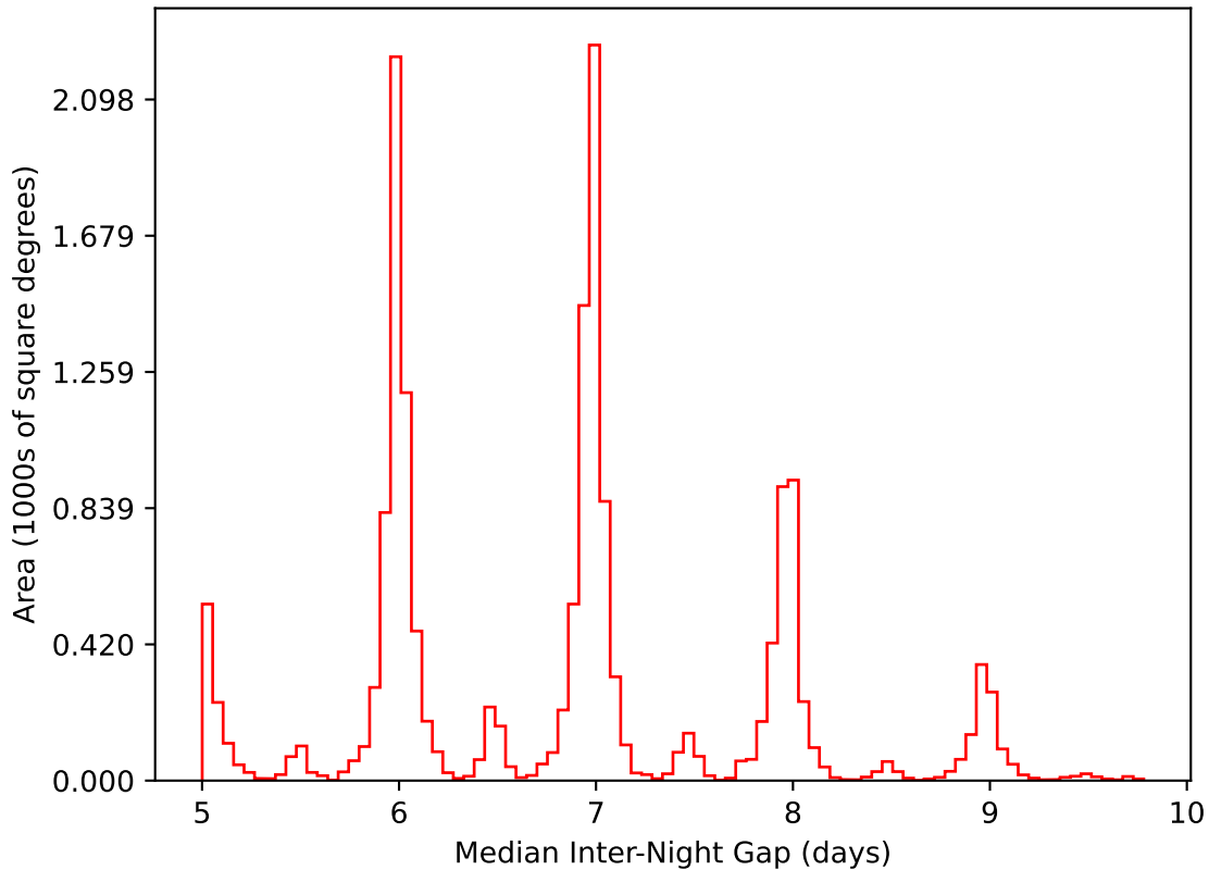
too_ignore_10_4v3.4_10yrs WFD i band: Median Inter-Night Gap
