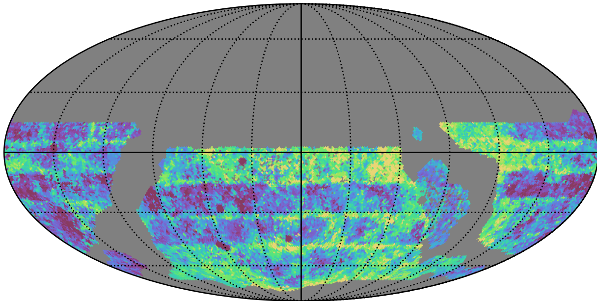
too_ignore_10_4v3.4_10yrs WFD g band: Median Inter-Night Gap
