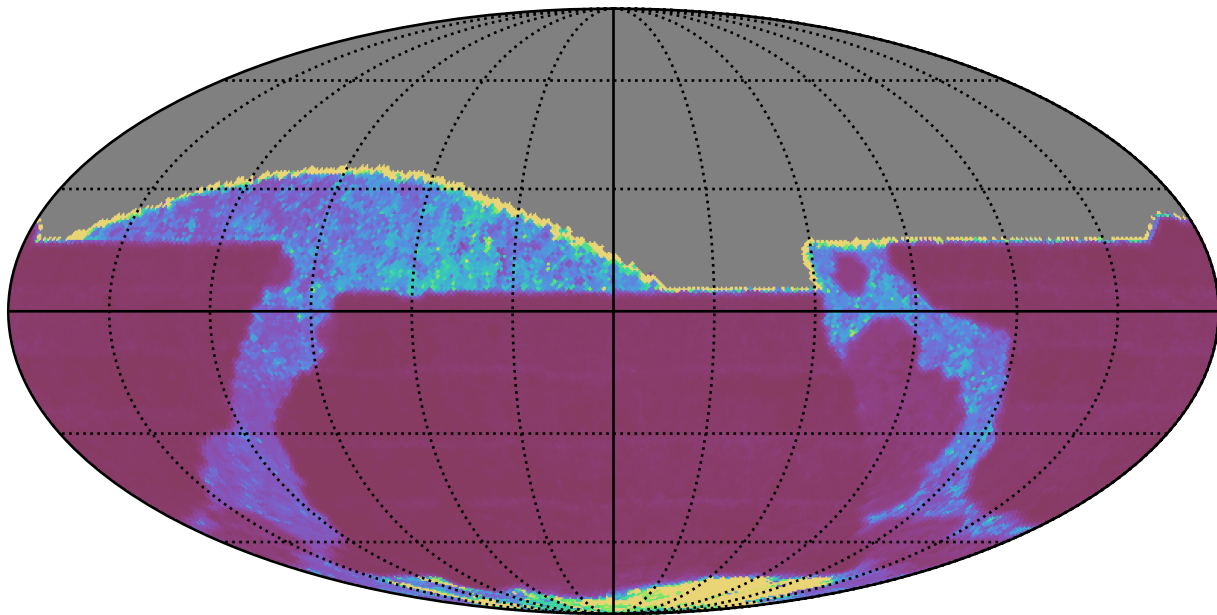
too_ignore_10_4v3.4_10yrs All sky z band: Median Inter-Night Gap
