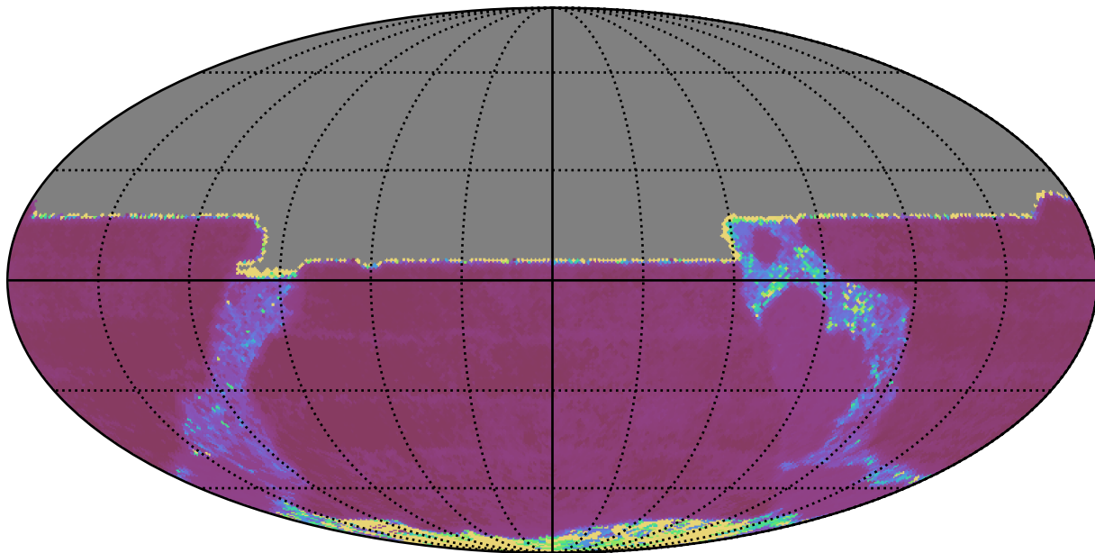
too_ignore_10_4v3.4_10yrs All sky y band: Median Inter-Night Gap
