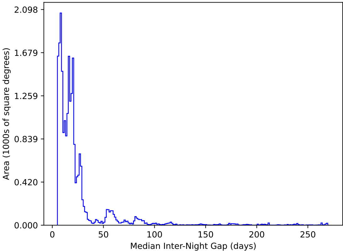
too_ignore_10_4v3.4_10yrs All sky y band: Median Inter-Night Gap
