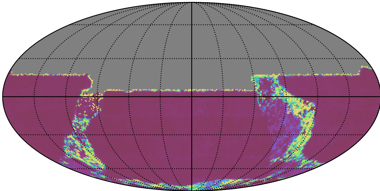
too_ignore_10_4v3.4_10yrs All sky u band: Median Inter-Night Gap
