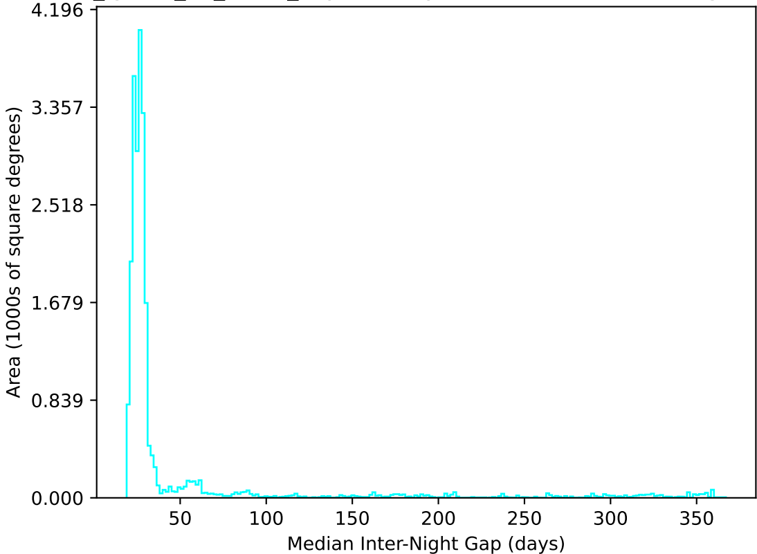
too_ignore_10_4v3.4_10yrs All sky u band: Median Inter-Night Gap
