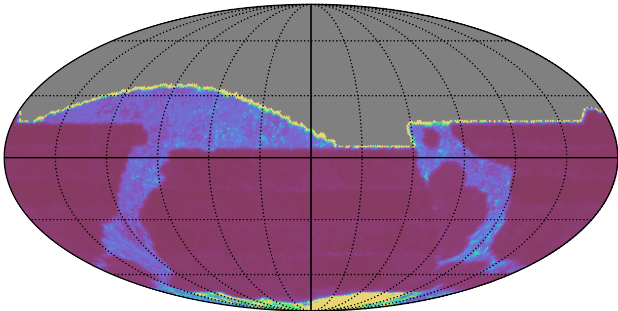
too_ignore_10_4v3.4_10yrs All sky r band: Median Inter-Night Gap
